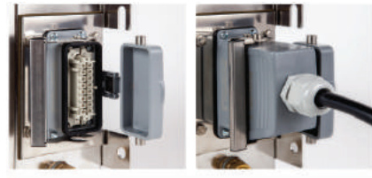
Example: Complete Cable Harness with Side "A" and "B" Connections
