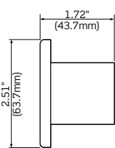
Female Protective Cap
