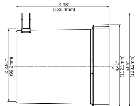
Panel Receptacle Housing
