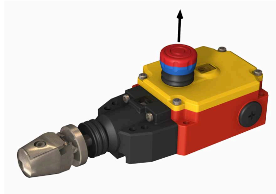
Figure 7: Resetting the latch
