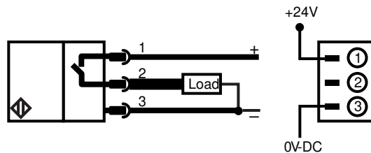
Figure 6: Warning signal electrical connections
