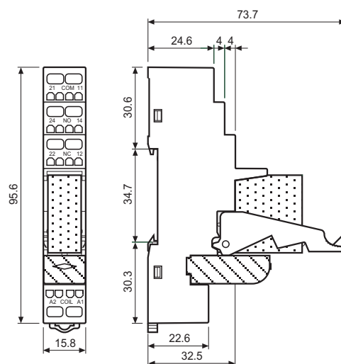
48.72 / 48.81 / 48.82 Screwless terminal
