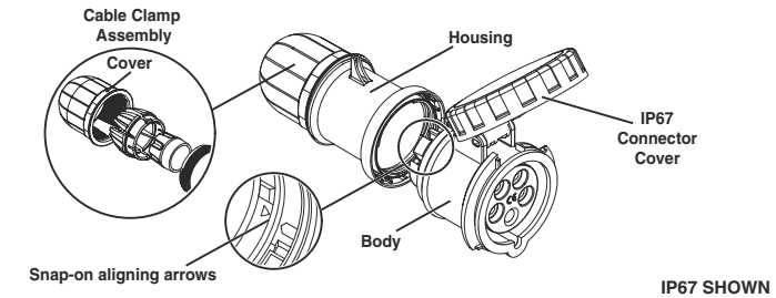
FIGURE 1: 16A & 32A IP67 CONNECTORS
