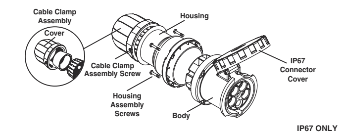
FIGURE 3: 63A & 125A IP67 CONNECTOR
