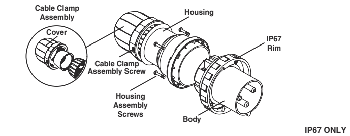
FIGURE 4: 63A & 125A IP67 PLUG
