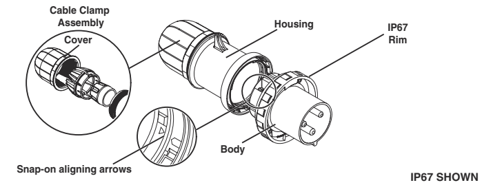
FIGURE 2: 16A & 32A IP67 PLUGS
