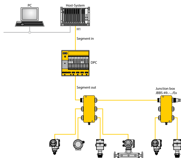
Fig. 2 Topology – FOUNDATION™ in the non-hazardous area
