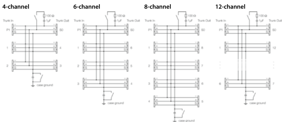
Terminal Connection
