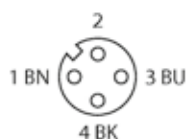
Male connector
