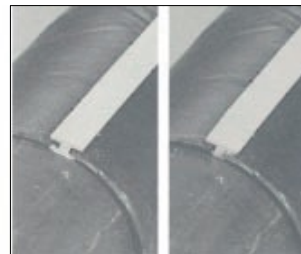
Seal with extruded H and T strips
