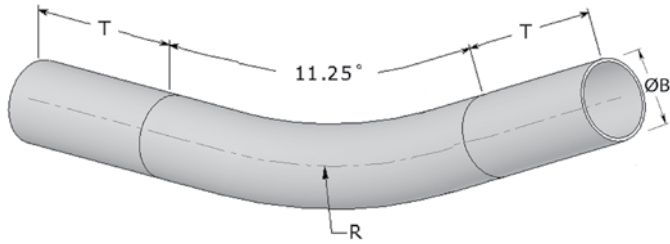
IPS HW 11.25° Elbow
