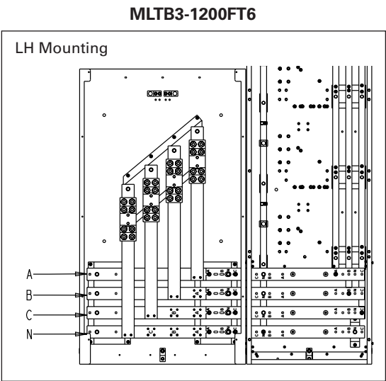
1200A feed-through tap box connections
