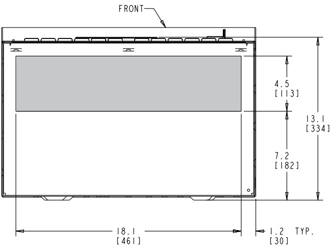
Bottom plate for 600V Meter stack - Inches (mm)
